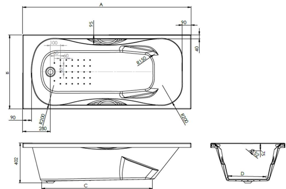
Technical drawing
