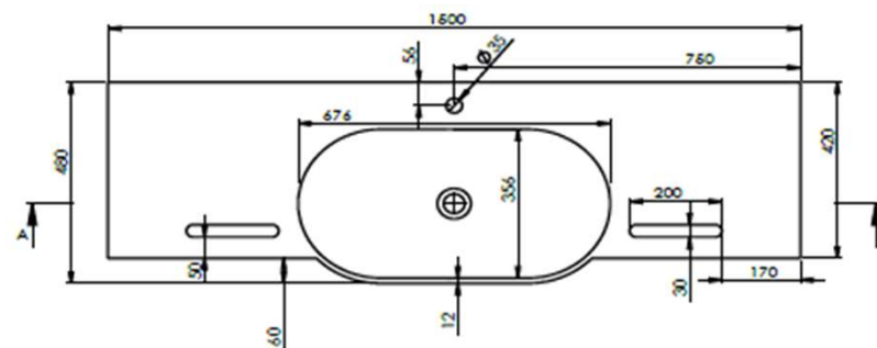
Technical drawing
