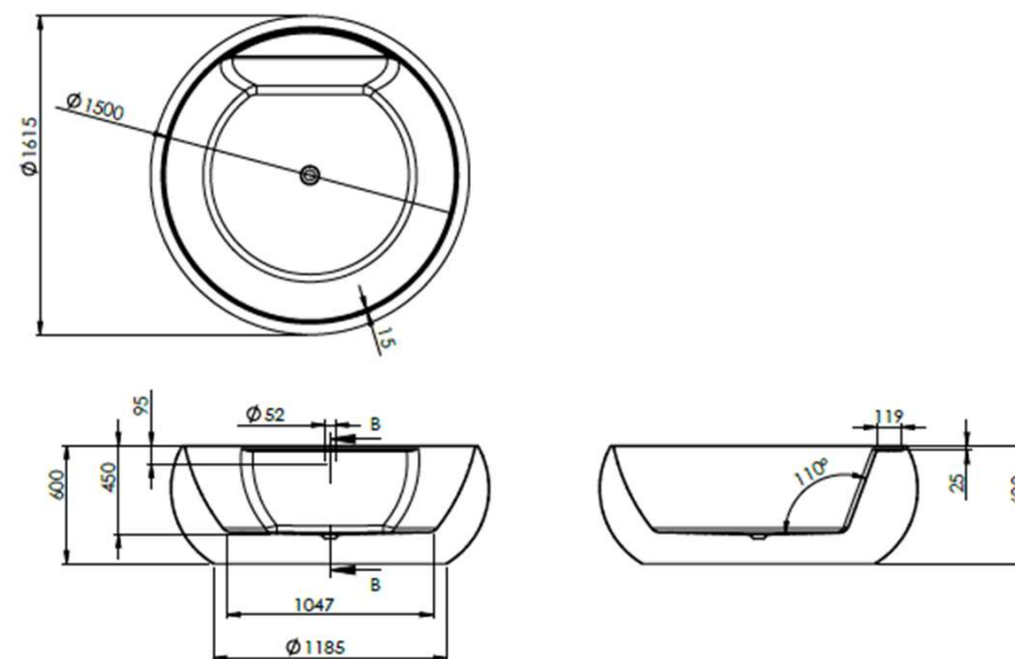
Technical drawing
