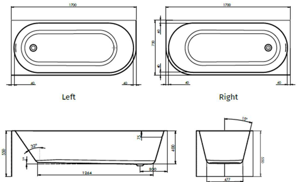
Technical drawing
